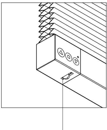
Bottom Sensor
